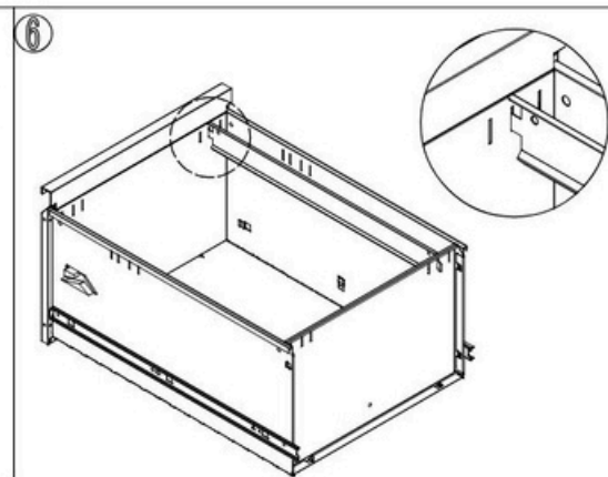
Fix the hanging rods with drawer panels as show in the picture.
